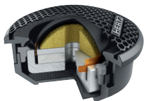
MP 25 3D cut-View
