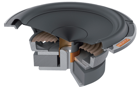
MP 165P.3 3D cut-View
