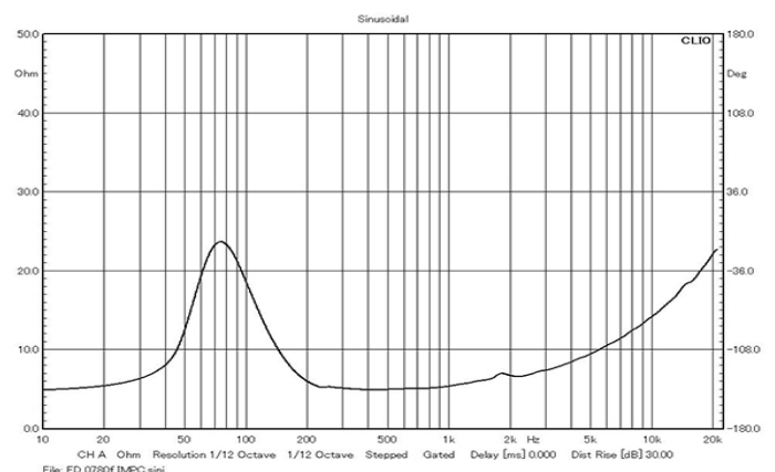
Impedance curve of FD 0780F
